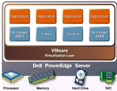
Figure 2. ESXi 5 architecture
