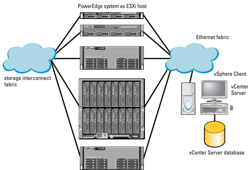
Figure 1. vSphere components
